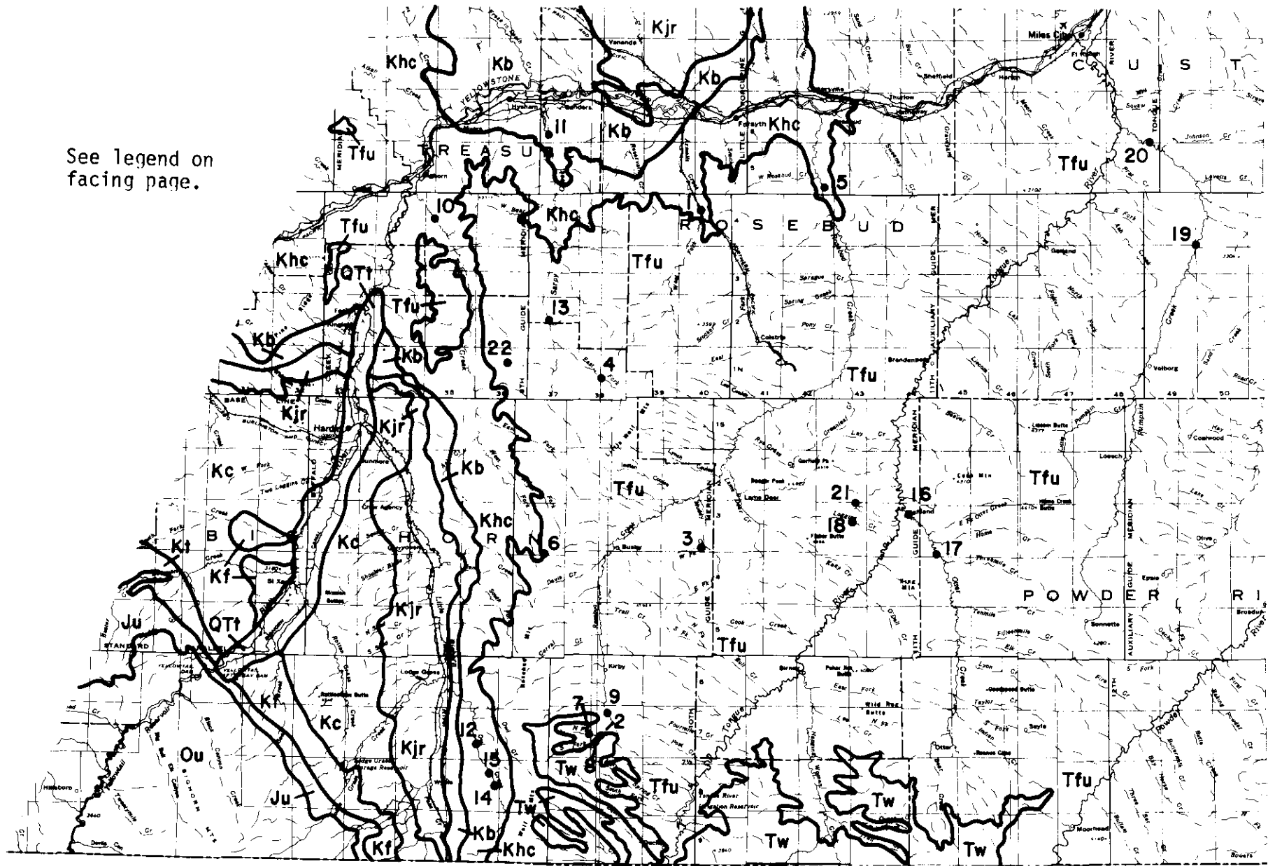
Figure 36. Generalized bedrock geology of southeastern Montana.
