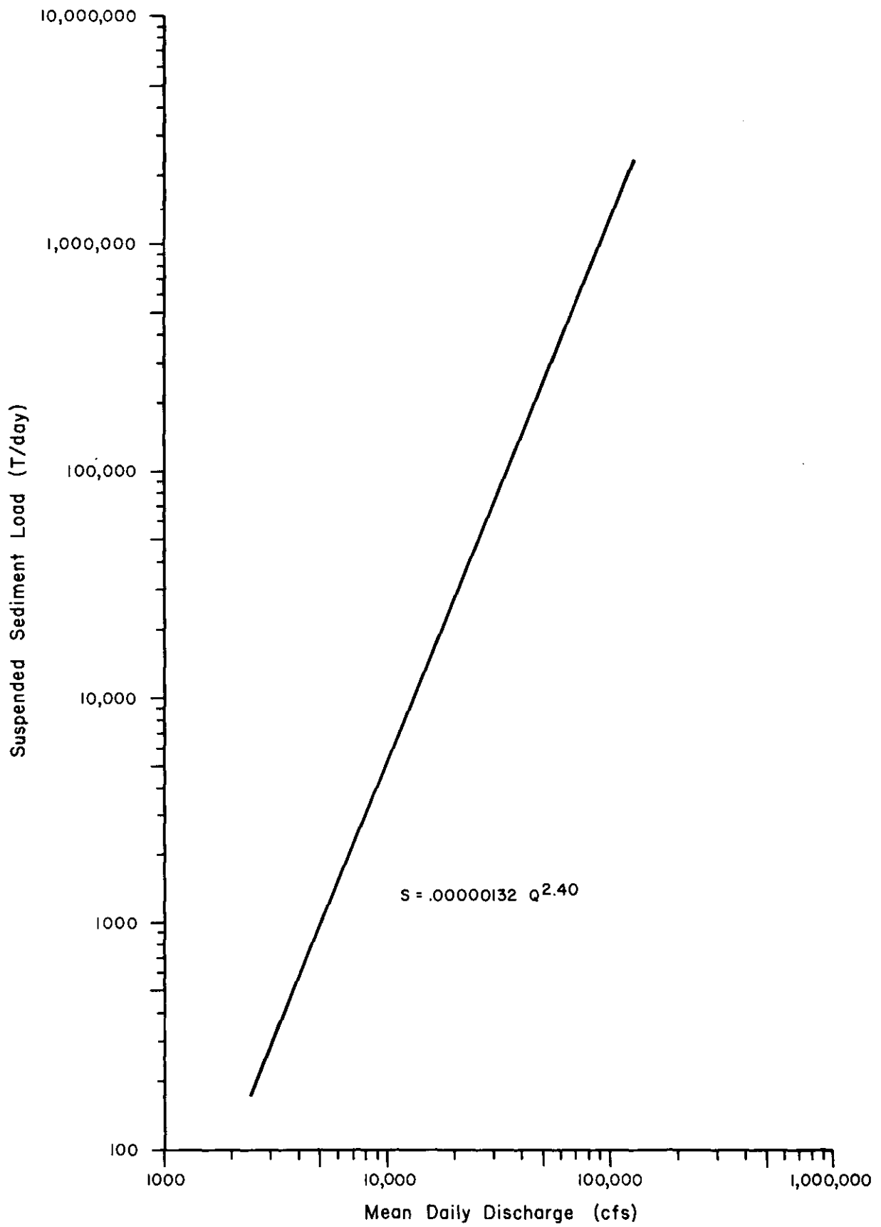
Figure 26. Suspended sediment load vs. discharge: Yellowstone River near Sidney.
