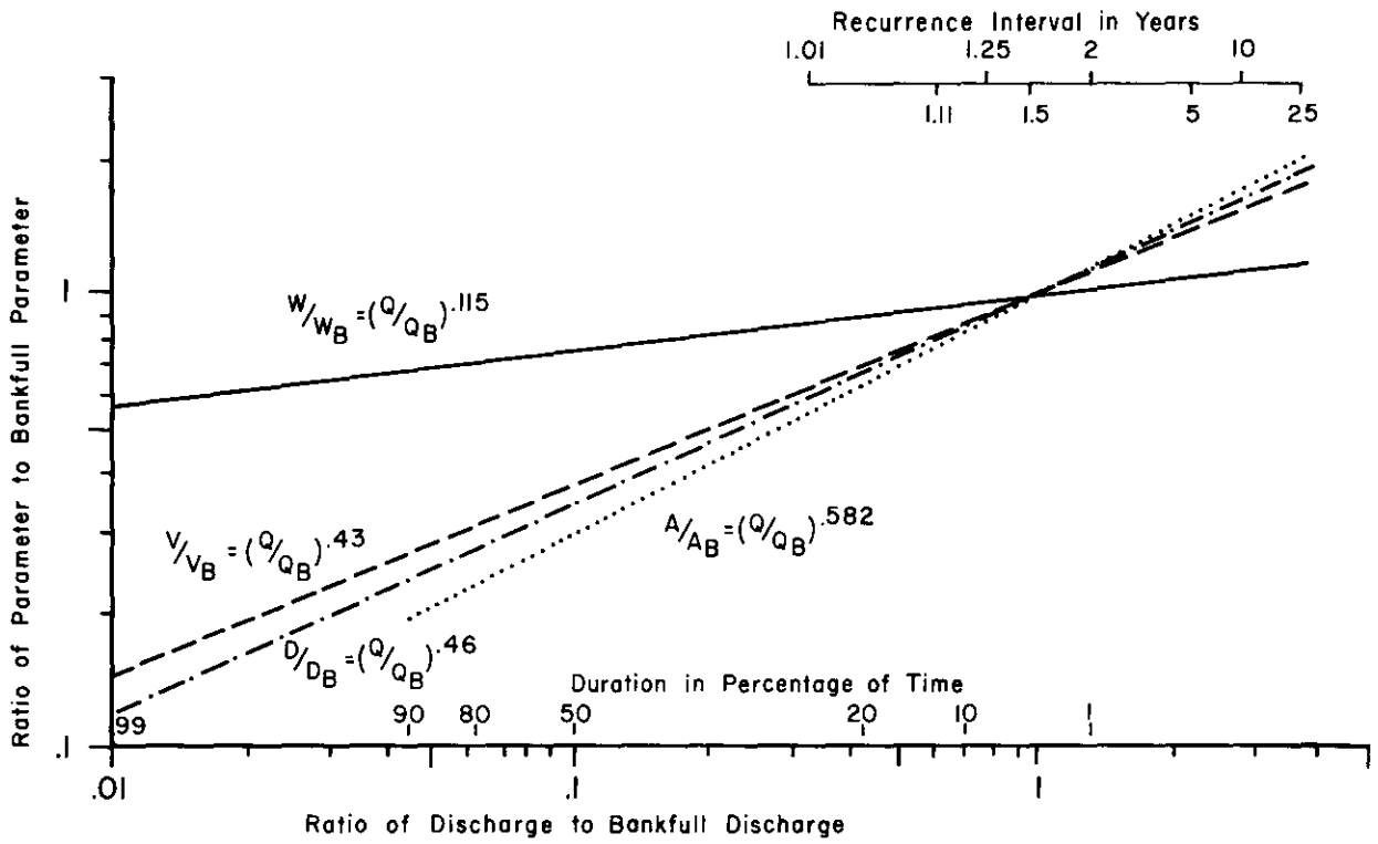
Figure 21. Dimensionless rating curve of the Tongue River.
