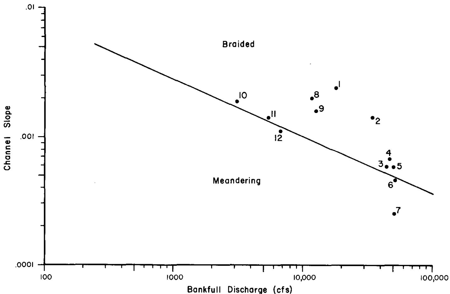
Figure 12. Relationship of rivers in the Yellowstone Basin to the general relation for channel form presented by Leopold and Wolman (1957).
