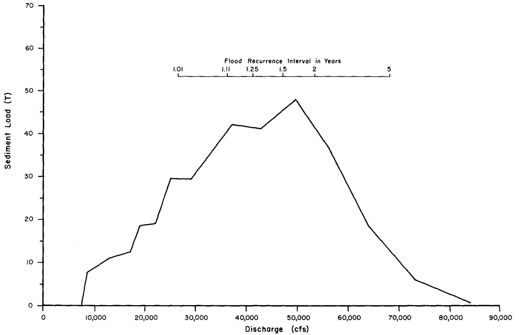
Figure 33. Sediment-duration curve showing most effective discharge: Yellowstone River at Miles City.
