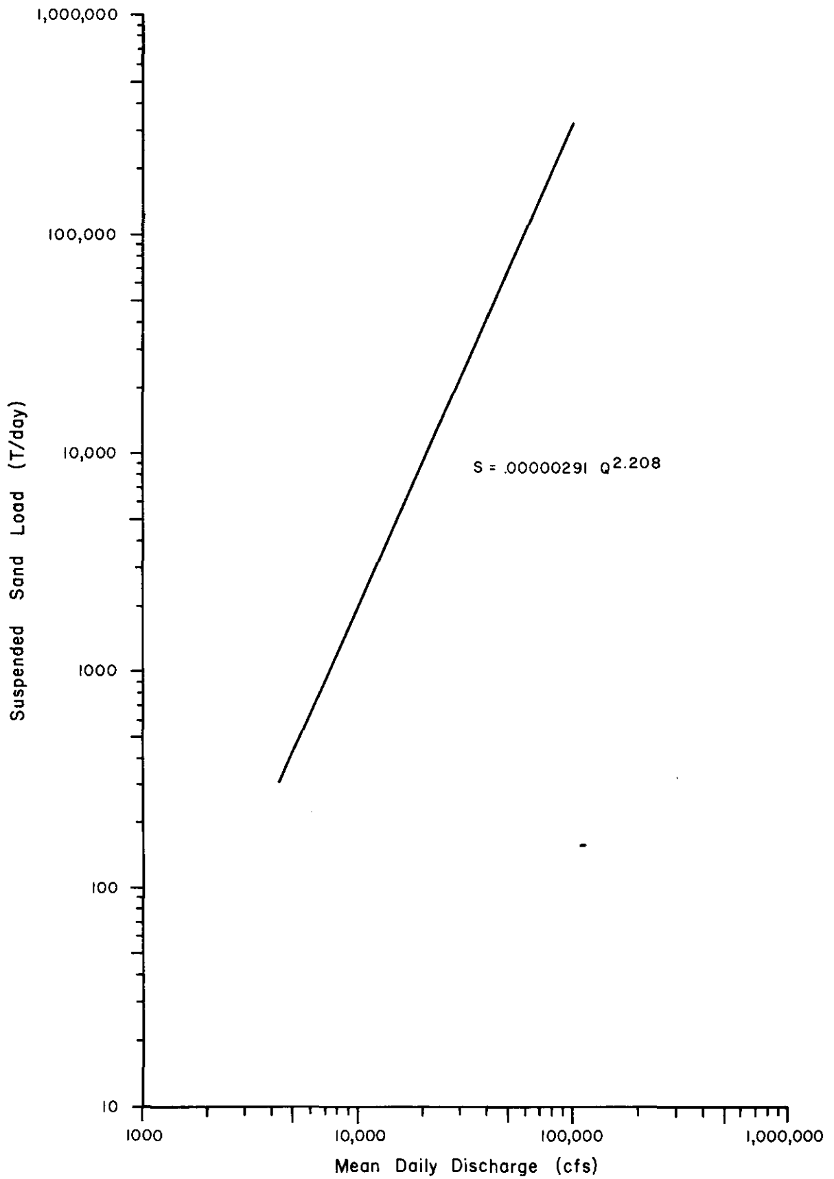
Figure 28. Suspended sand load vs. discharge: Yellowstone River near Sidney.
