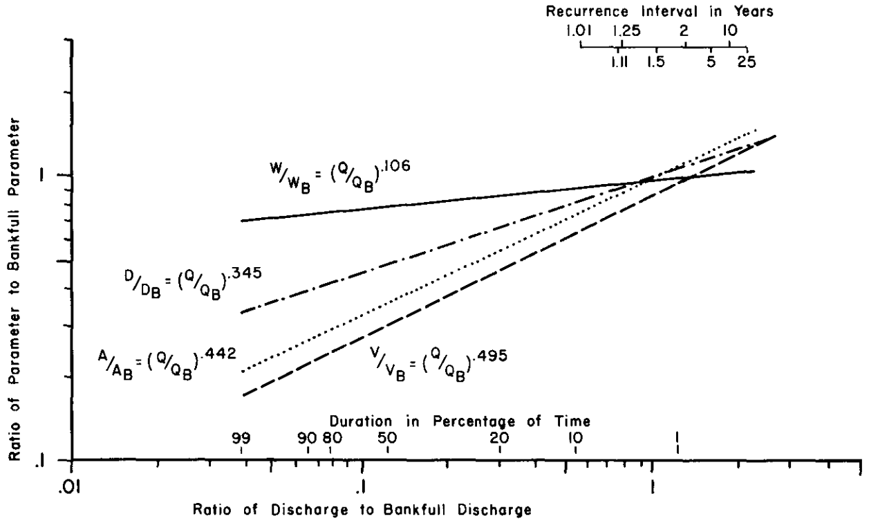
Figure 19. Dimensionless rating curve of the Yellowstone mainstem.
