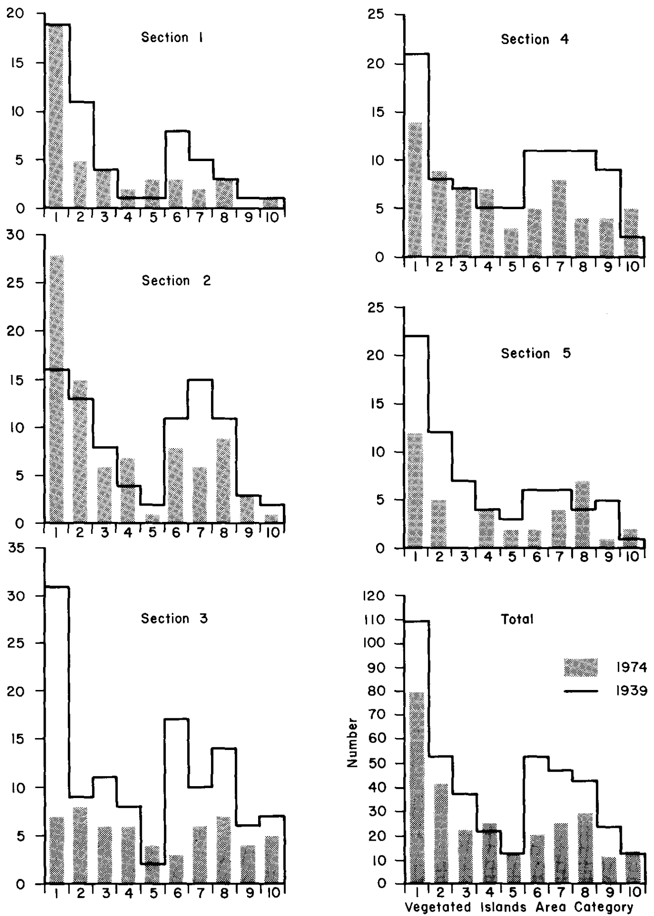
Figure B-1. Vegetated islands on the Bighorn River by area categories prior to and after Yellowtail Dam.
