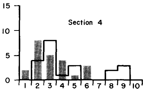
Figure B-3. Absolute numbers of lateral gravel bars on the Bighorn River by area categories prior to and after Yellowtail Dam.
