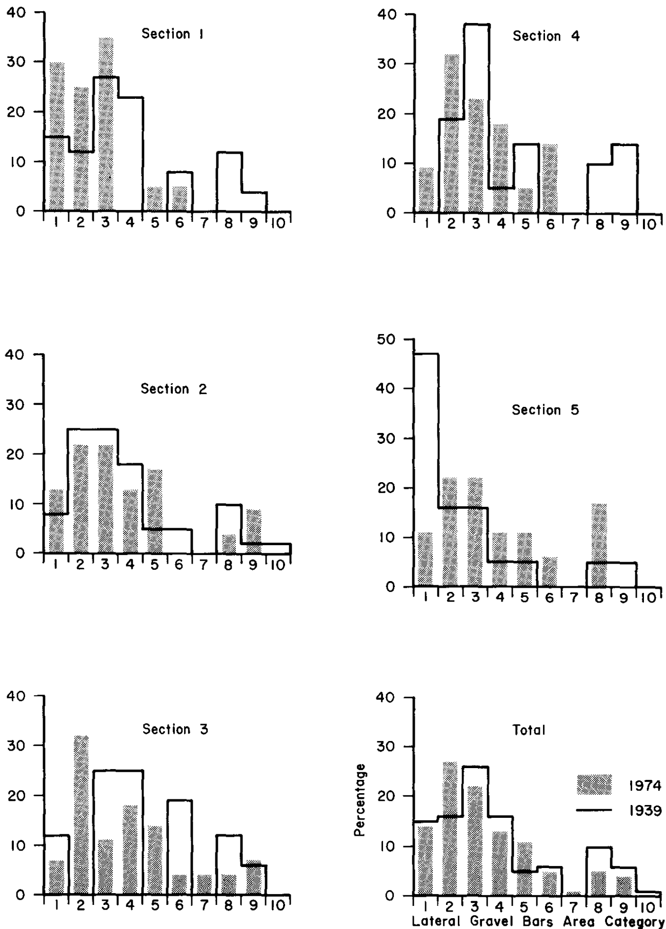
Figure B-6. Percentages of lateral gravel bars on the Bighorn River by area categories prior to and after Yellowtail Dam.
