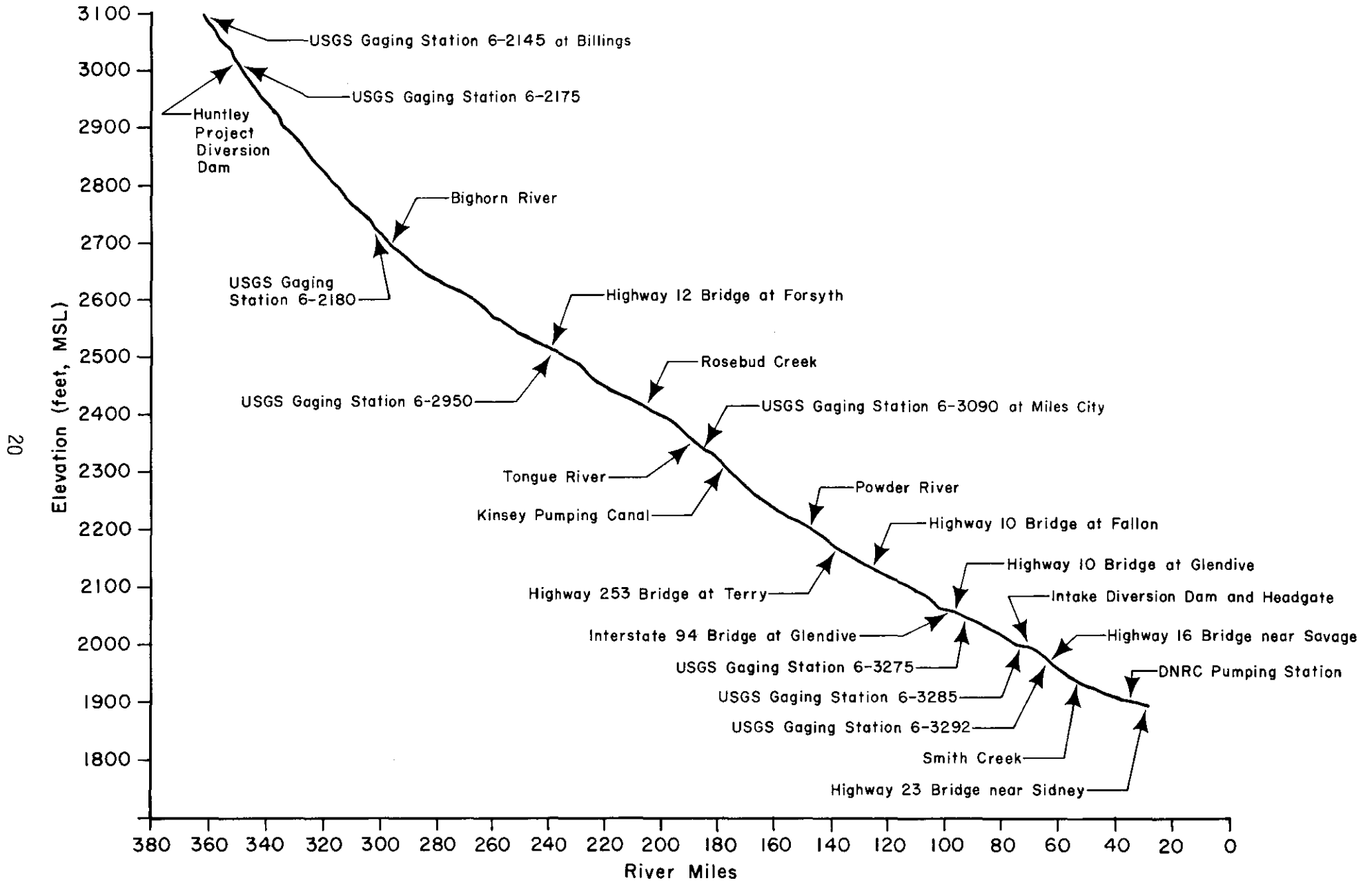
Figure 3. Profile of the Yellowstone River Mainstem between Billings and Sidney.
