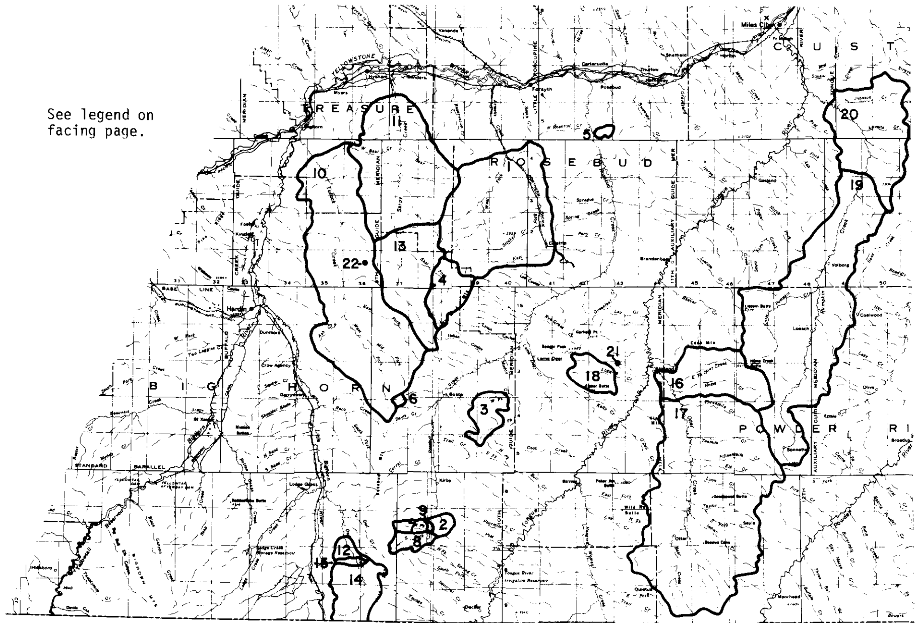
Figure 35. Vigil network stations in southeastern Montana and the approximate boundaries of the watersheds monitored.
