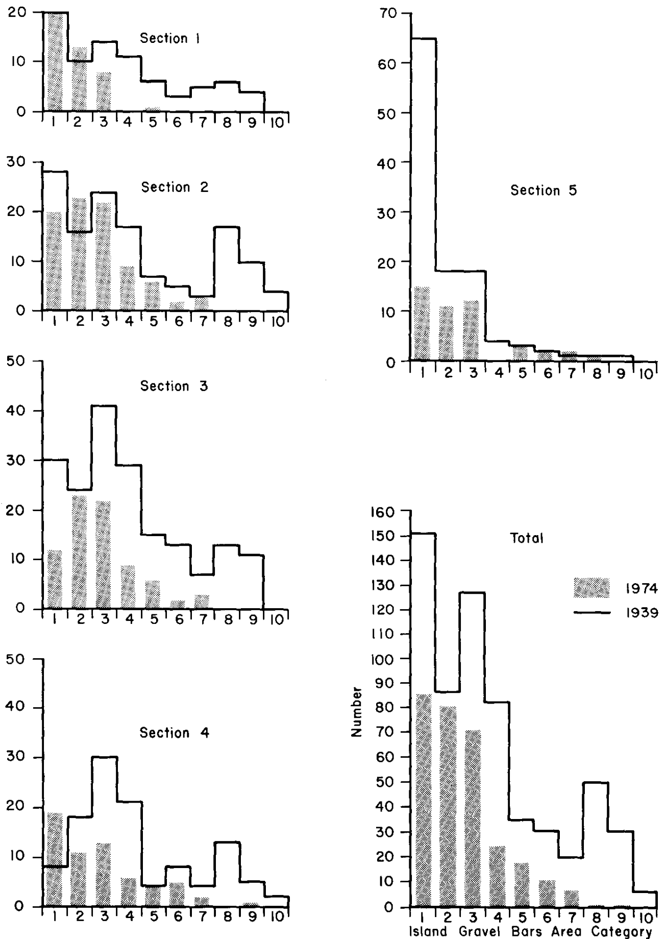
Figure B-2. Island gravel bars on the Bighorn River by area categories prior to and after Yellowtail Dam.
